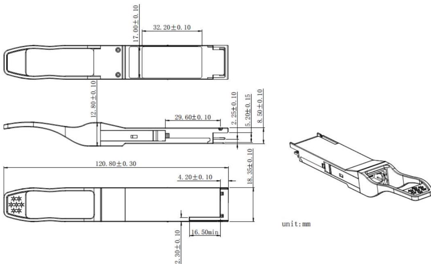
Figure10. Mechanical Specifications
