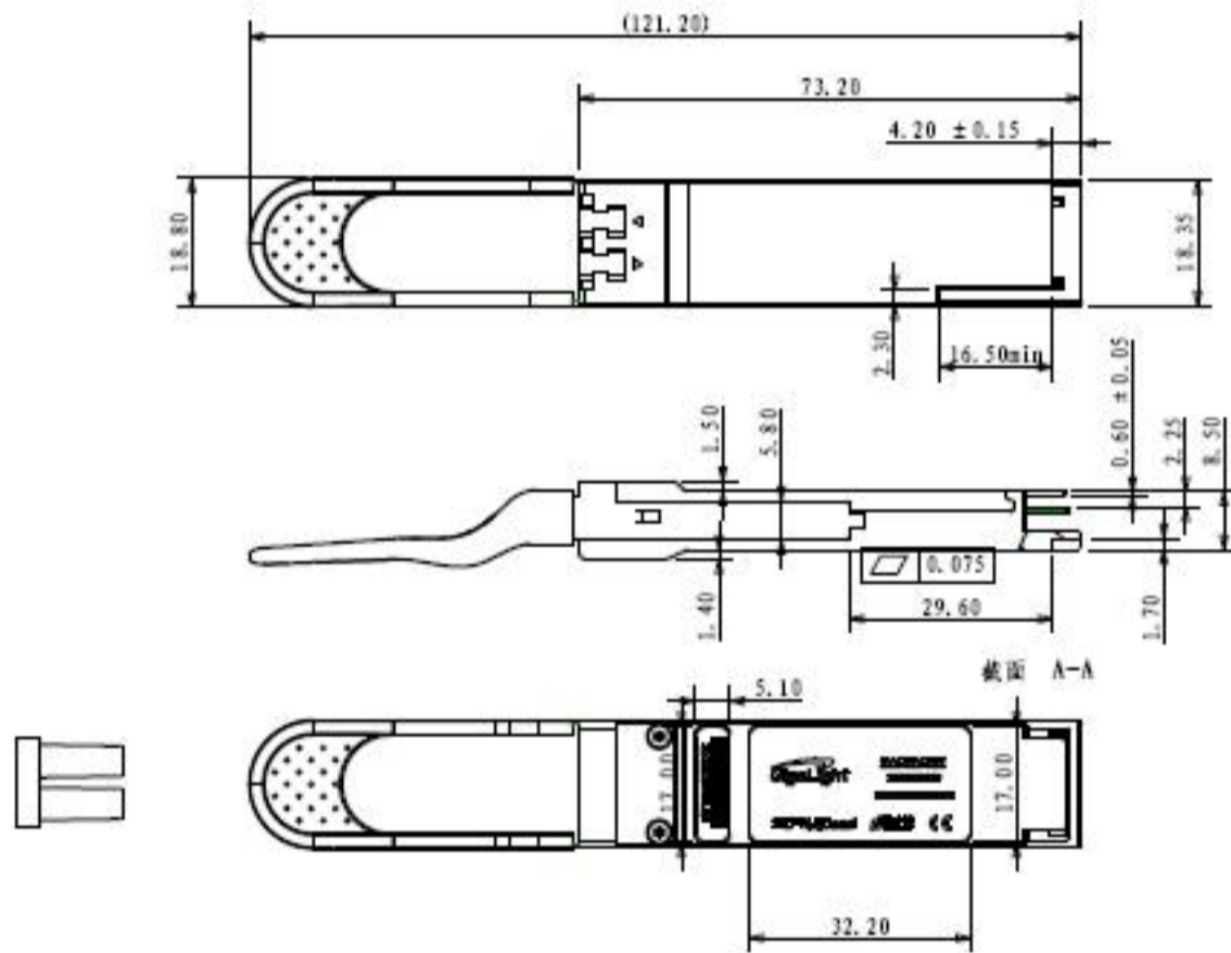
Figure10.Mechanical Specifications
