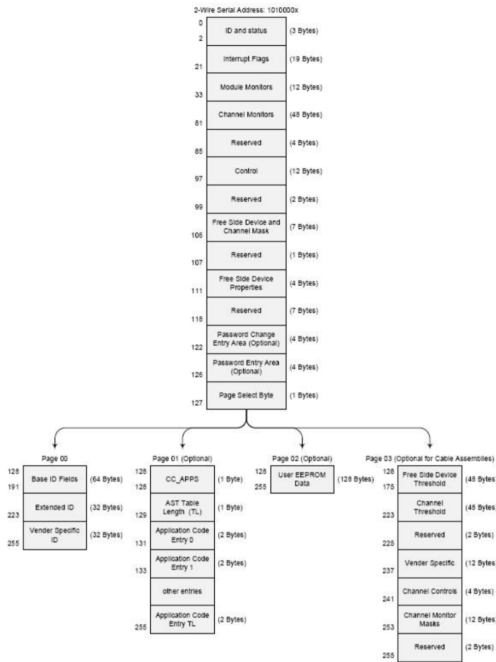
Figure5.QSFP Memory Map
