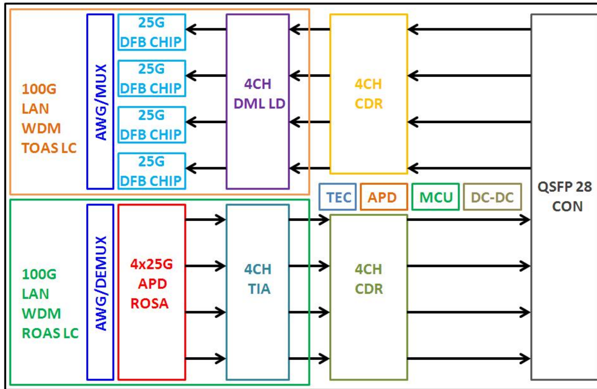
Figure1.Module Block Diagram
