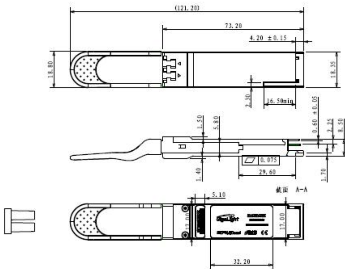
Figure10.Mechanical Specifications
