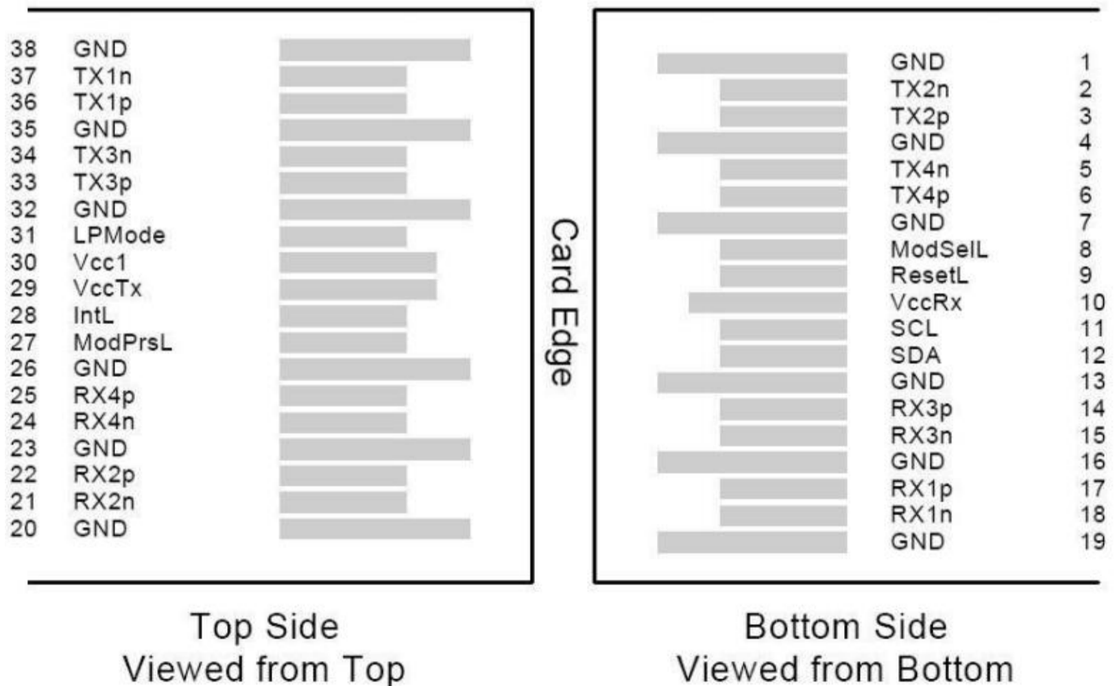
Figure 3. Pad Layout of the QSFP28connector
