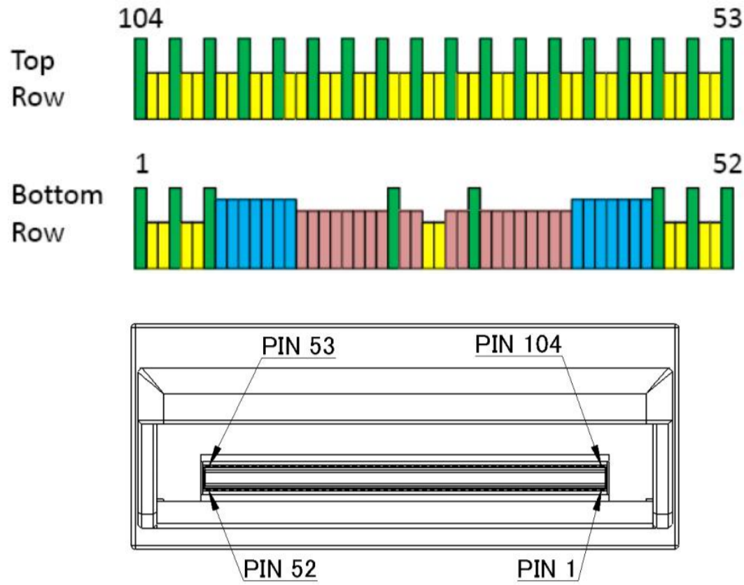
Figure2.Pad Layout of the CFP connector
