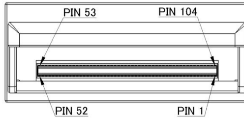
Pad Layout of the CFP2 module
