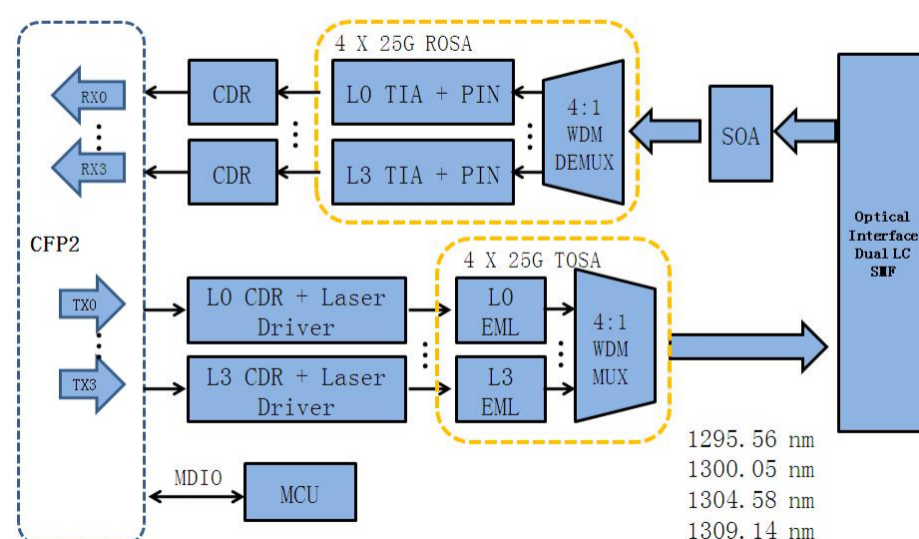
100GE CFP2 ER4 Module Block Diagram
