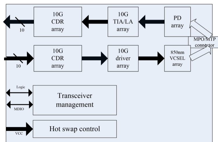
Figure1.Module Block Diagram
