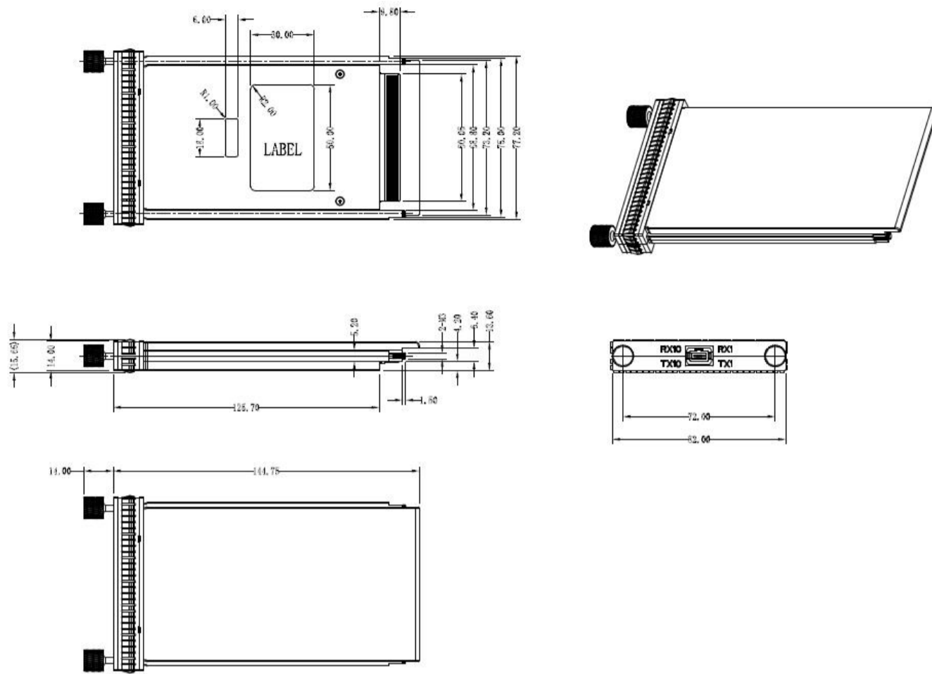
Figure 5. Mechanical Specifications
