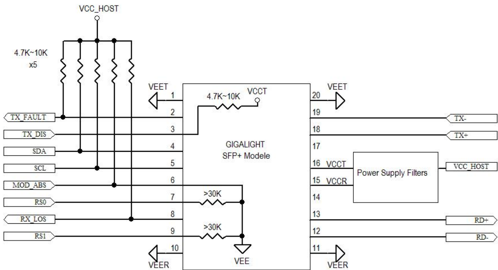
Figure4. Host-Module Interface
