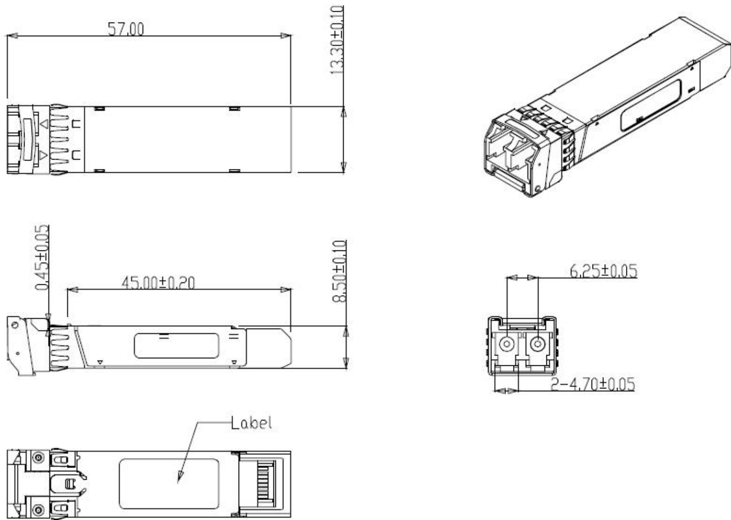
Figure5. Mechanical Specifications
