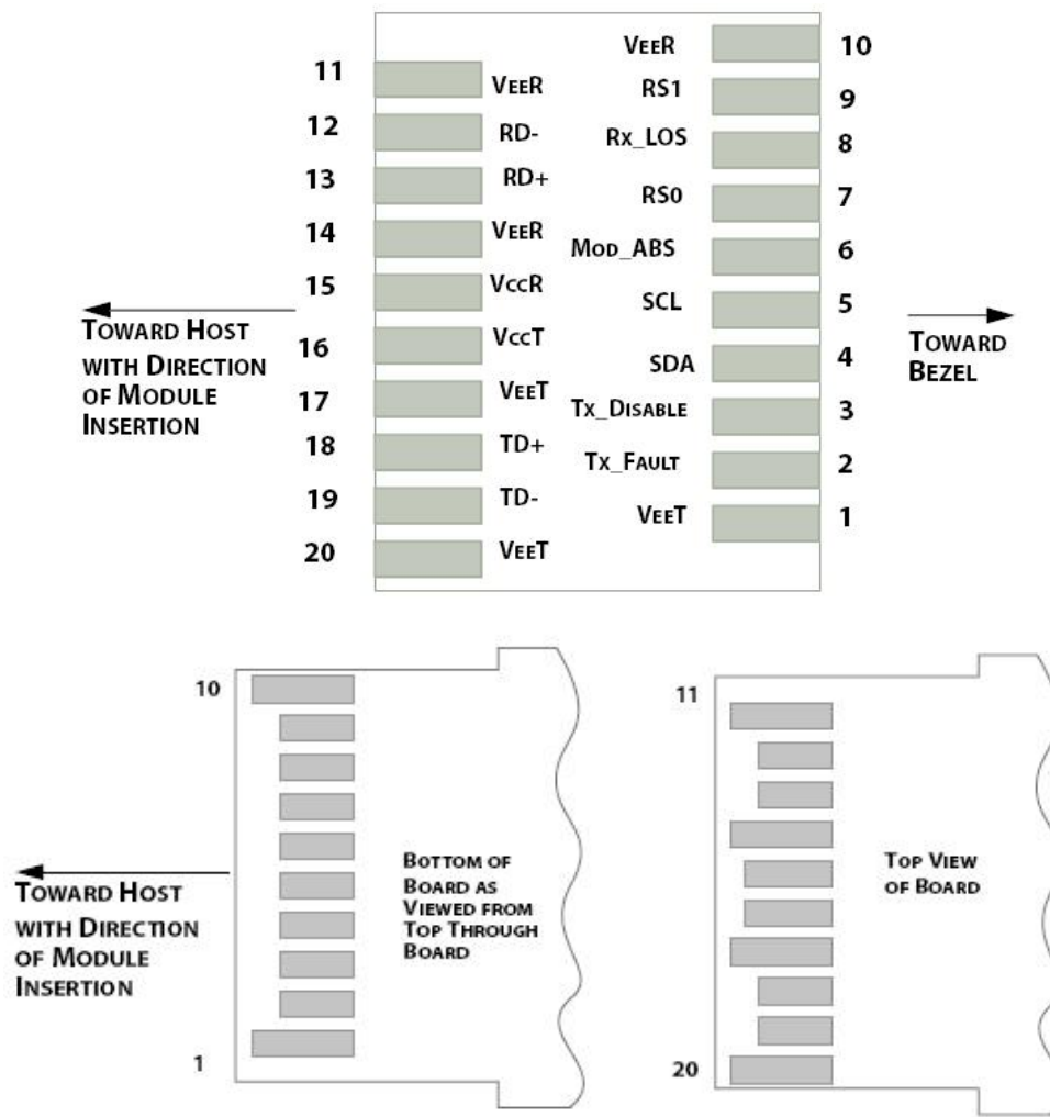
Figure2. Electrical Pin-out Details
