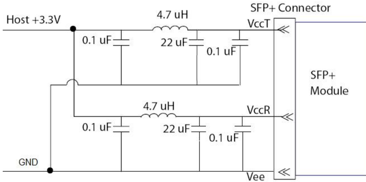
Figure3. Host Board Power Supply Filters Circuit
