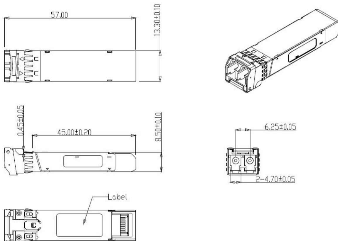
Figure5. Mechanical Specifications
