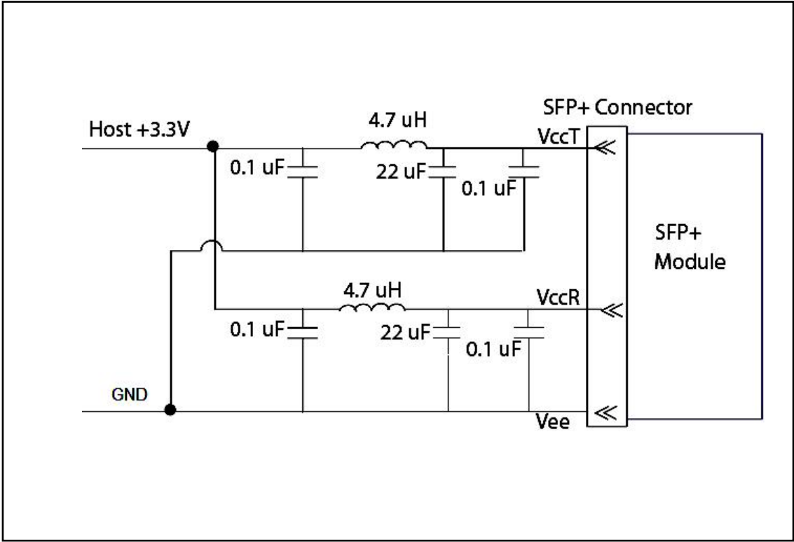
Figure2. Host Board Power Supply Filters Circuit
