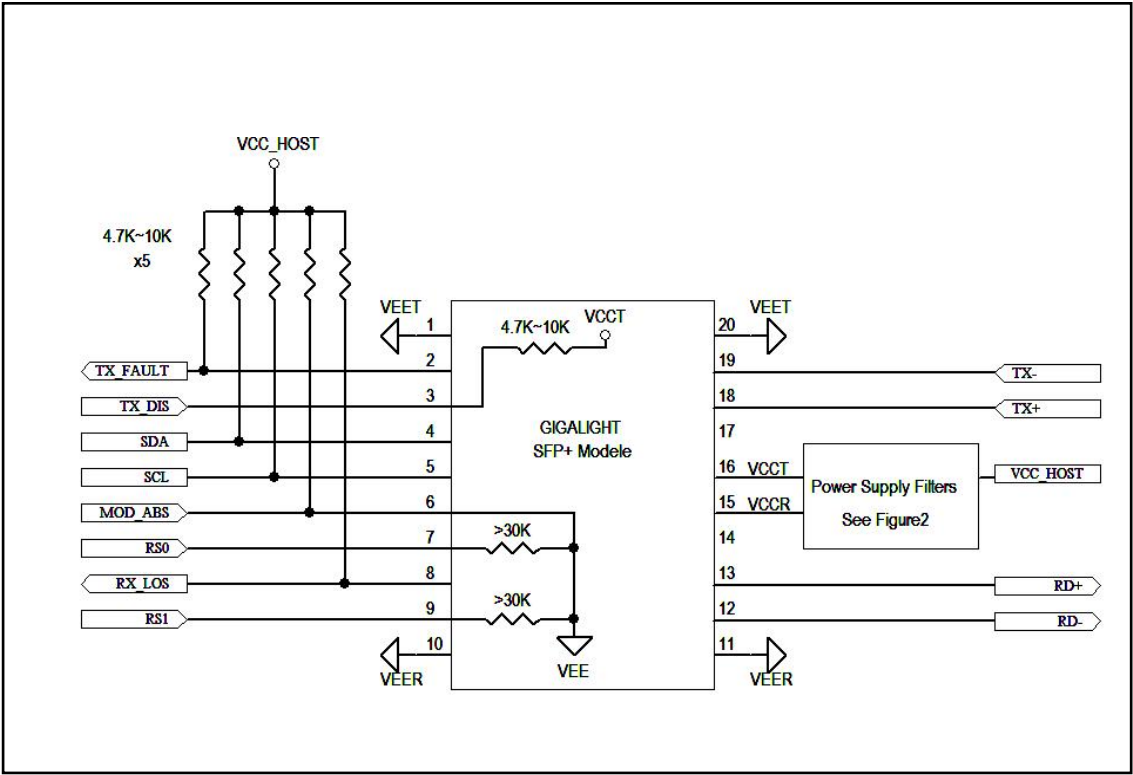
Figure3. Host-Module Interface
