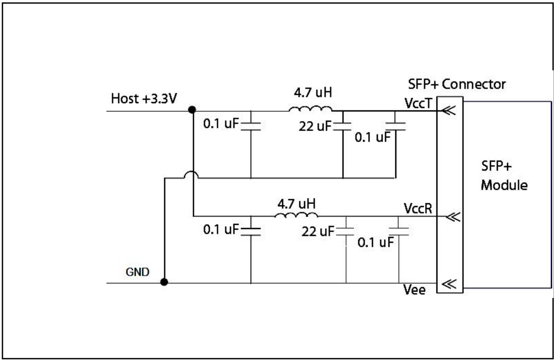
Figure2. Host Board Power Supply Filters Circuit
