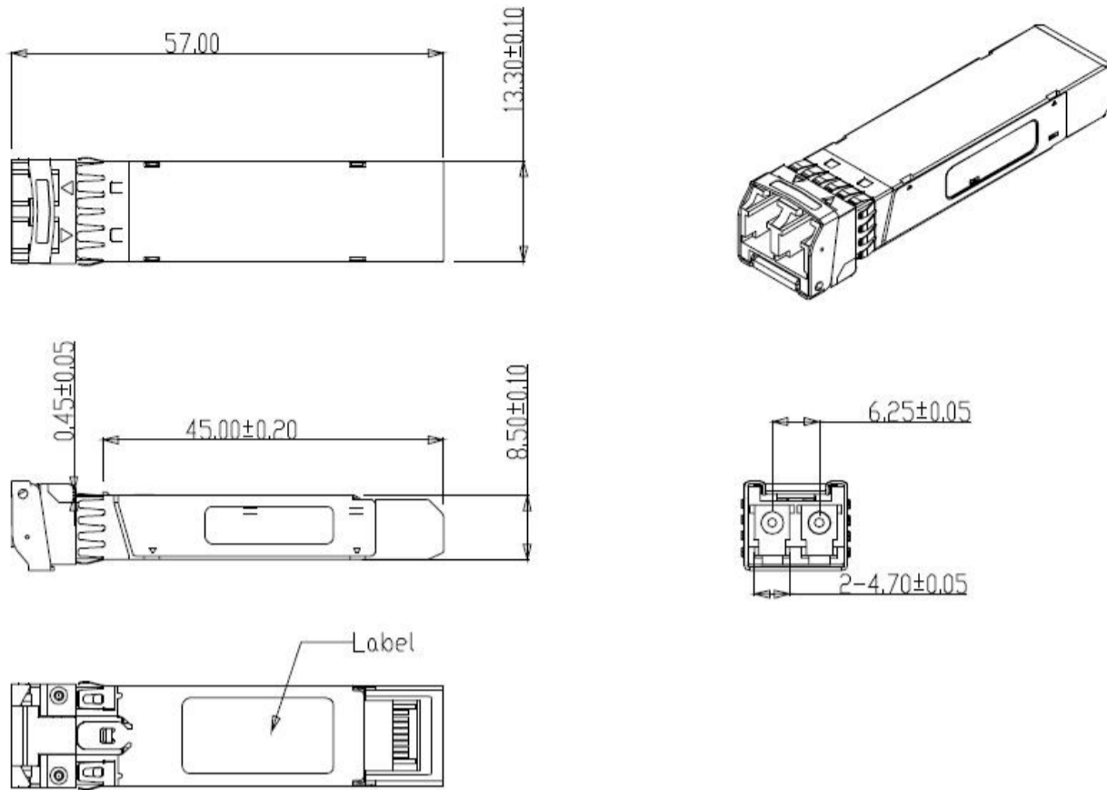
Figure5. Mechanical Specifications
