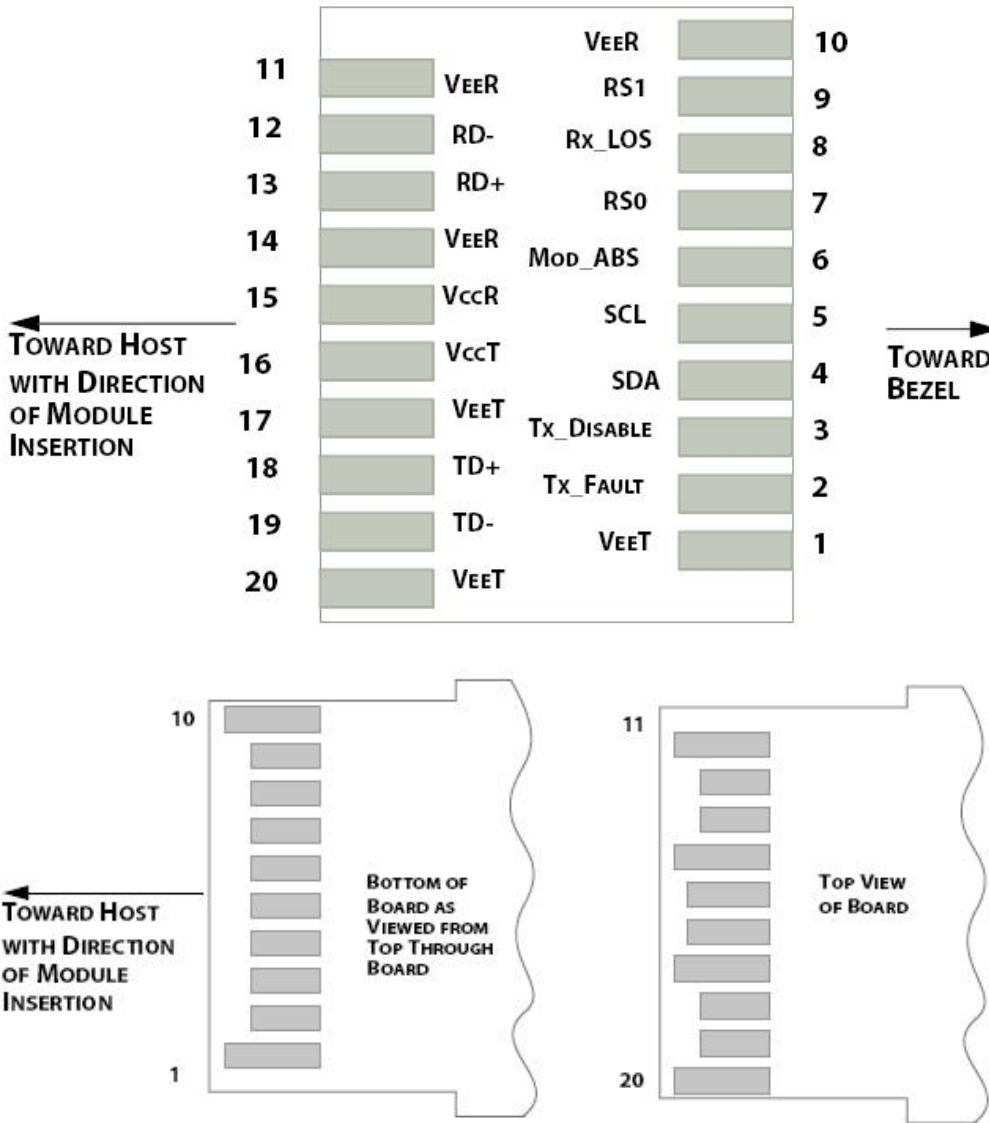
Figure2.Electrical Pin-out Details
