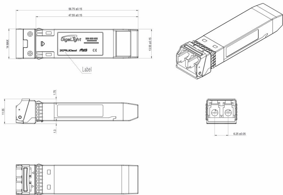
Figure5. Mechanical Specifications
