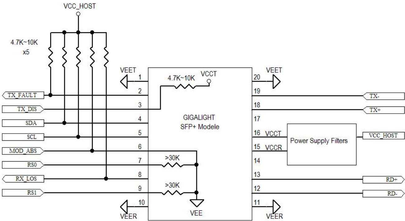
Figure4. Host-Module Interface
