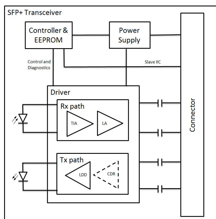
Figure1. Module Block Diagram
