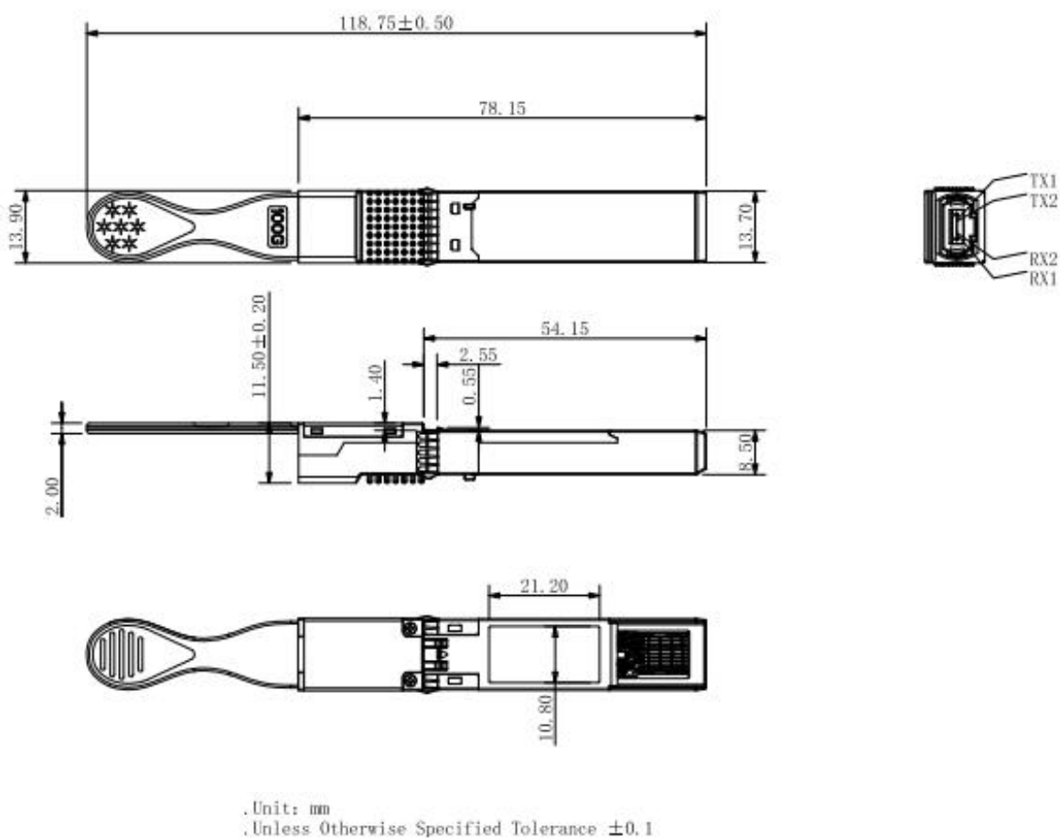
Figure 12. Mechanical Specifications
