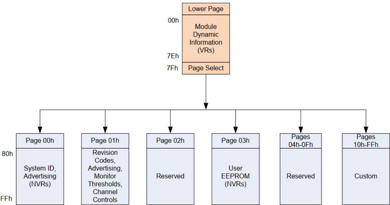
Figure 5. SFP-DD MIS Module Memory Map
