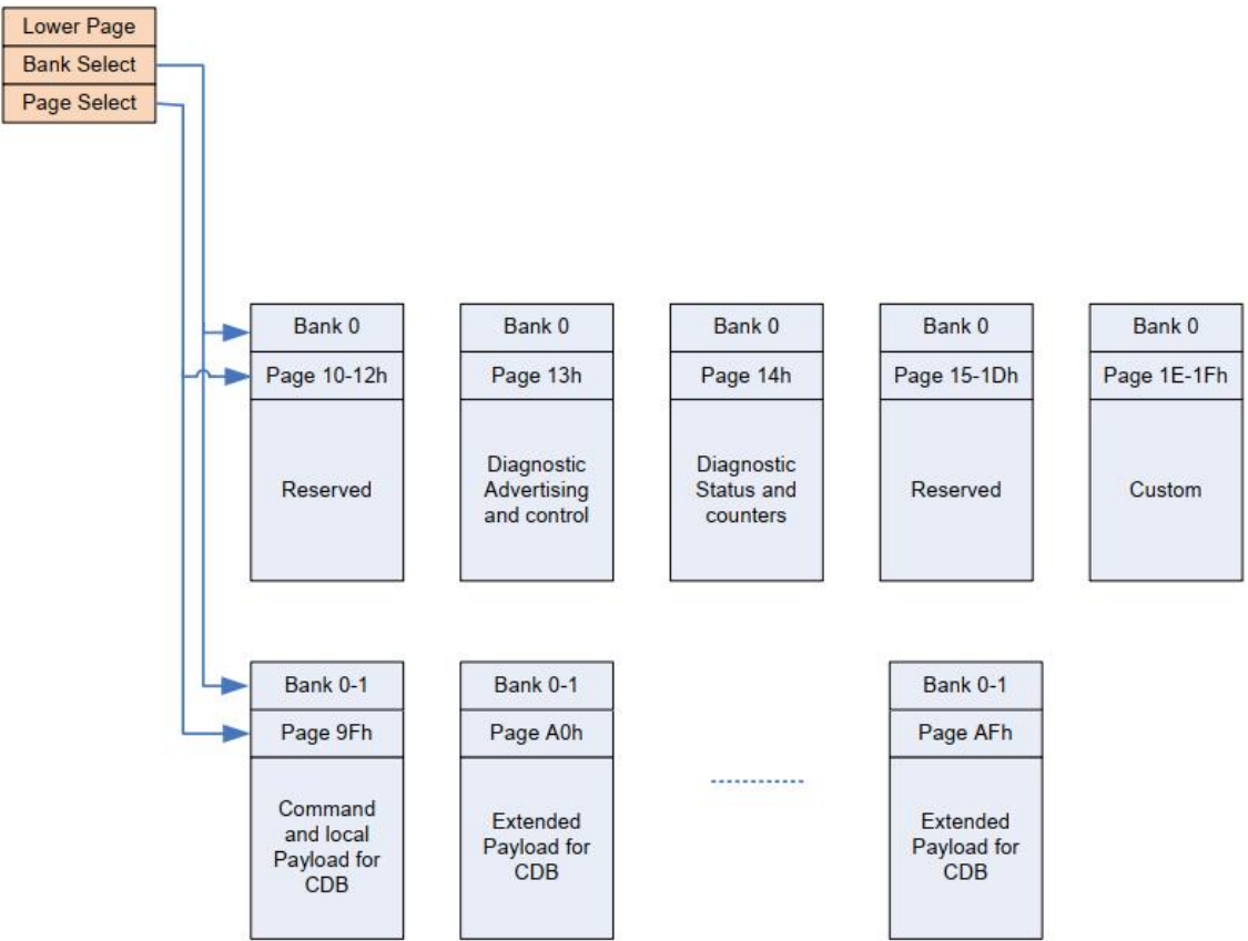
Figure 6. SFP-DD MIS Bank Page Memory Map
