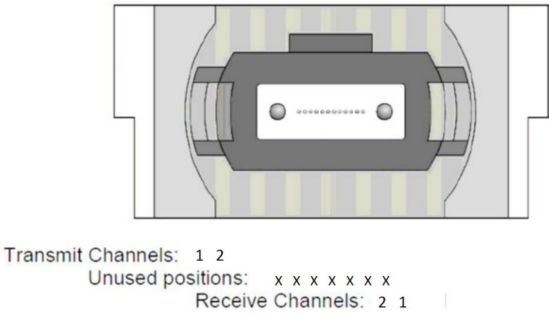
Figure 4. Optical Receptacle and Channel Orientation
