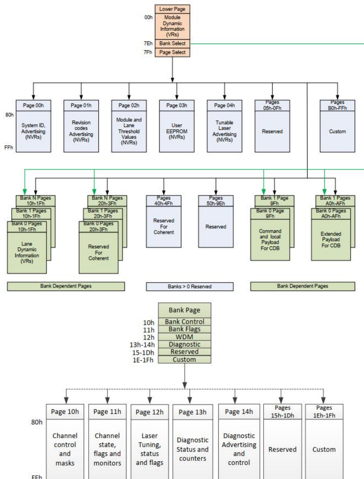
Figure 2. SFP112 Memory Map
