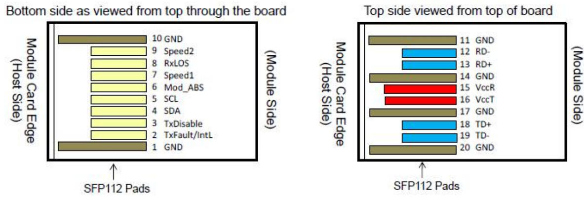
Figure 3. Pin View
