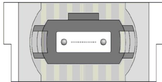
Transmit Channels: 1 2 3 4 Unused positions: X X X X Receive Channels: 4 3 2 1
