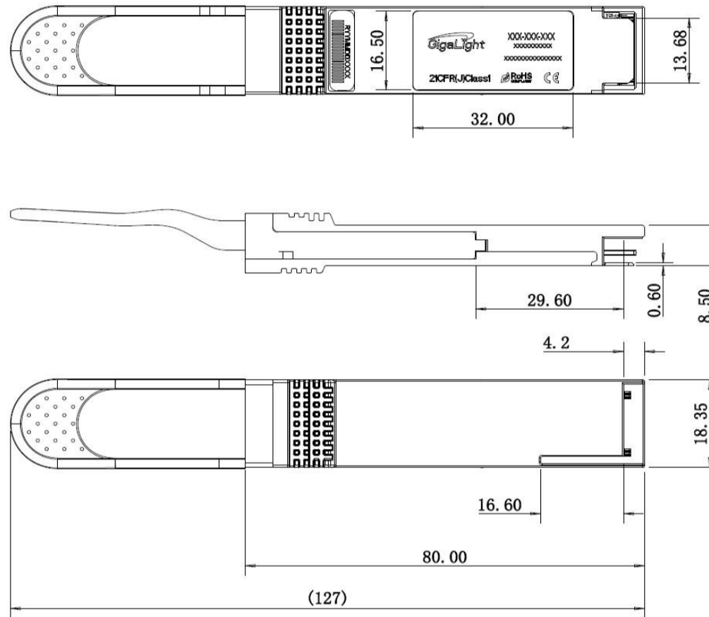
Figure10. Mechanical Specifications
