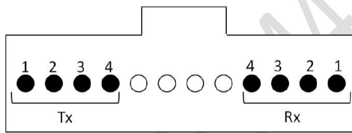
Figure 4. Optical Receptacle and Channel Orientation
