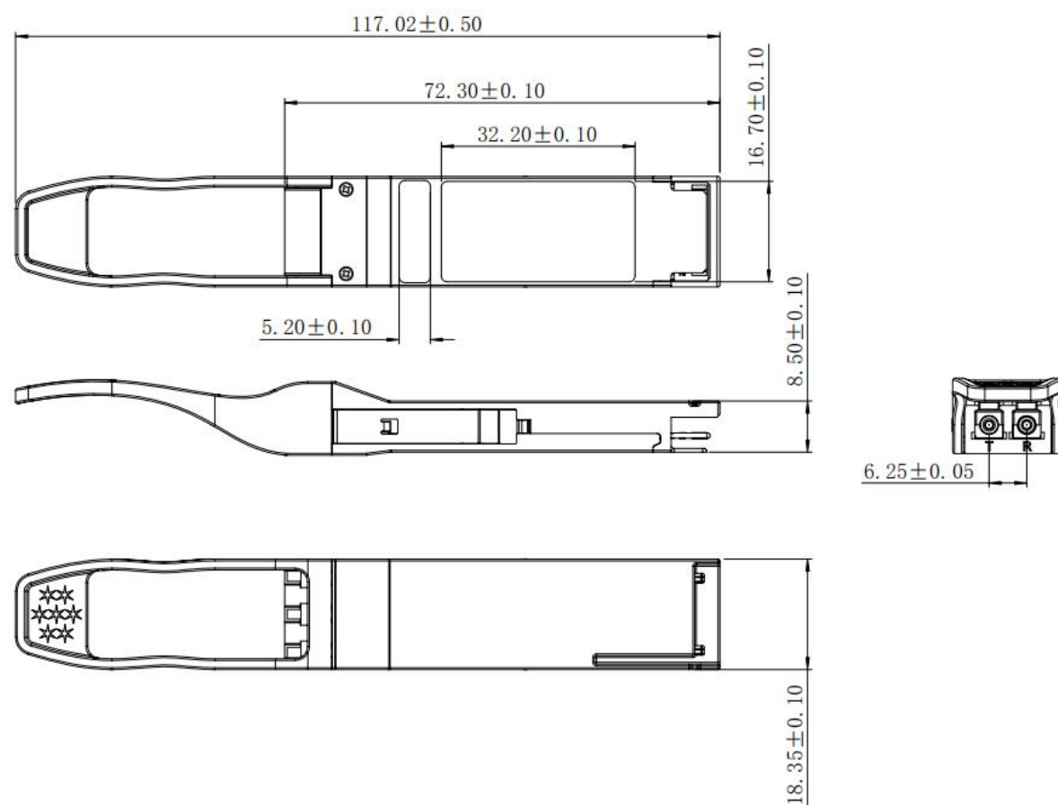
Figure 9. Mechanical Specifications
