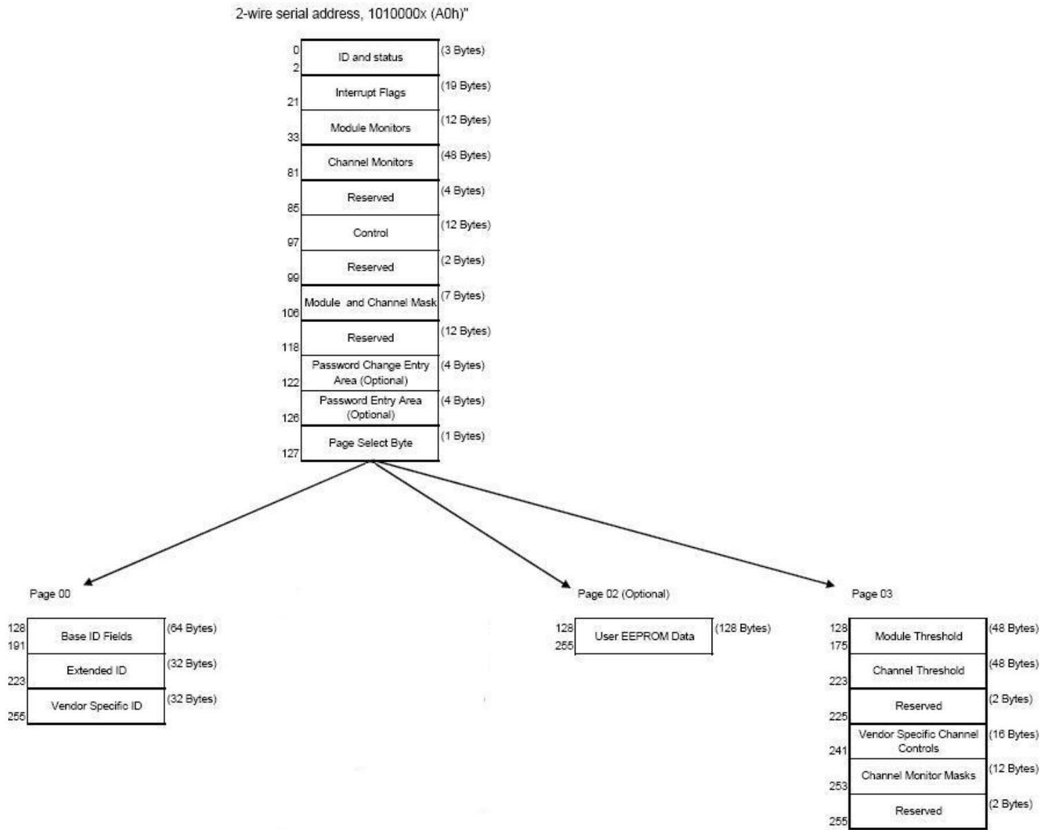
Figure 4. QSP28 Memory Map
