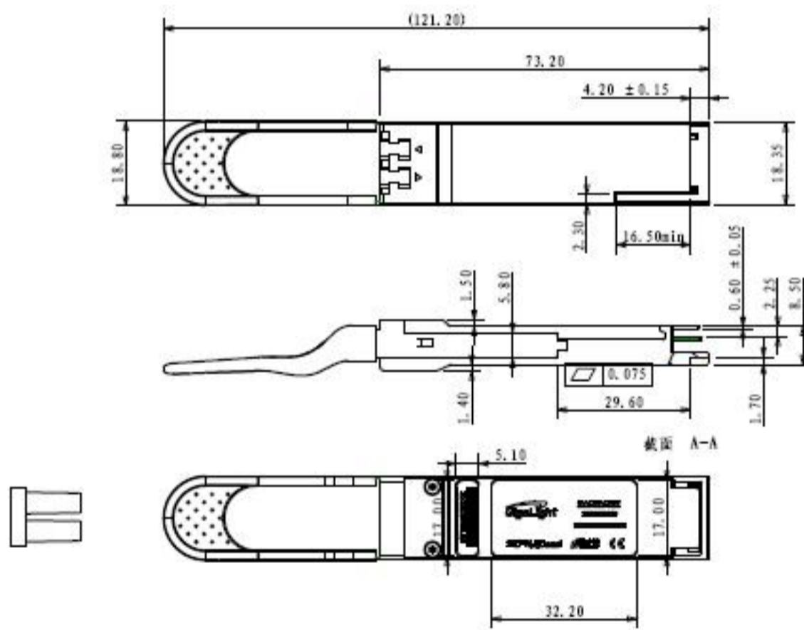
Figure7.Mechanical Specifications
