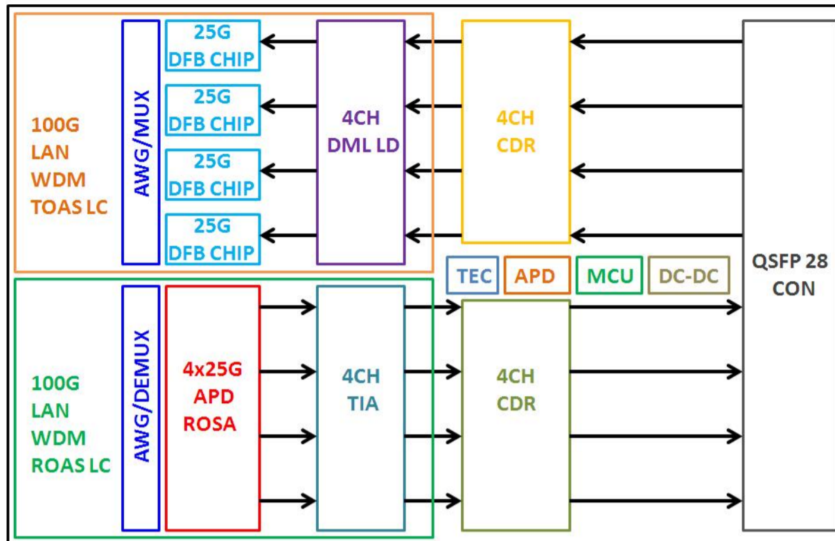
Figure1.Module Block Diagram
