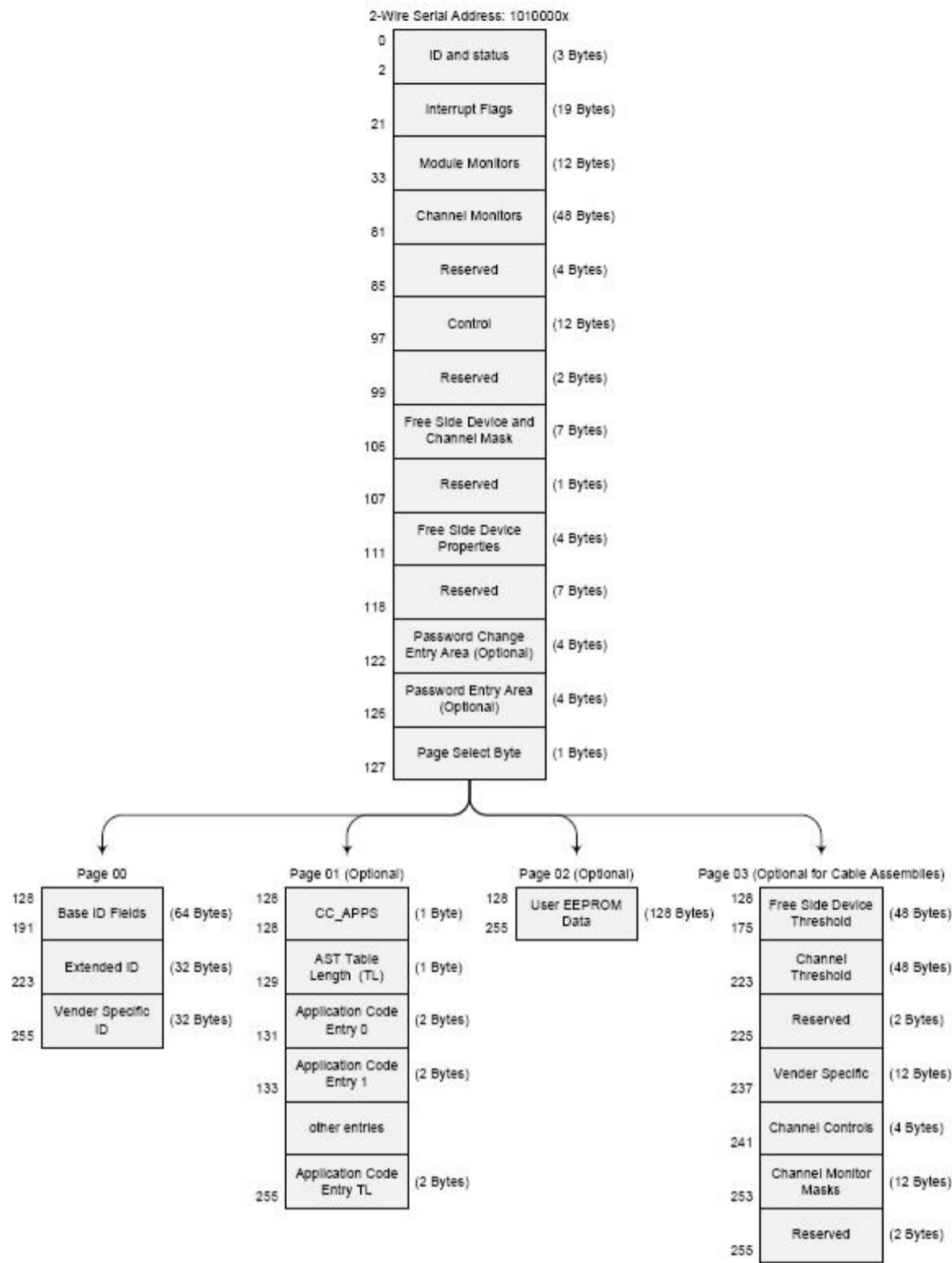
Figure3.QSFP Memory Map
