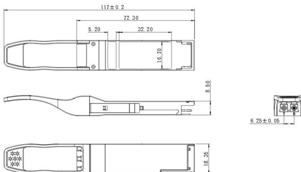
Figure 8. Mechanical Specifications
