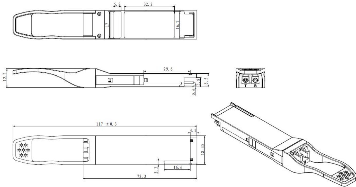
Figure 8. Mechanical Specifications
