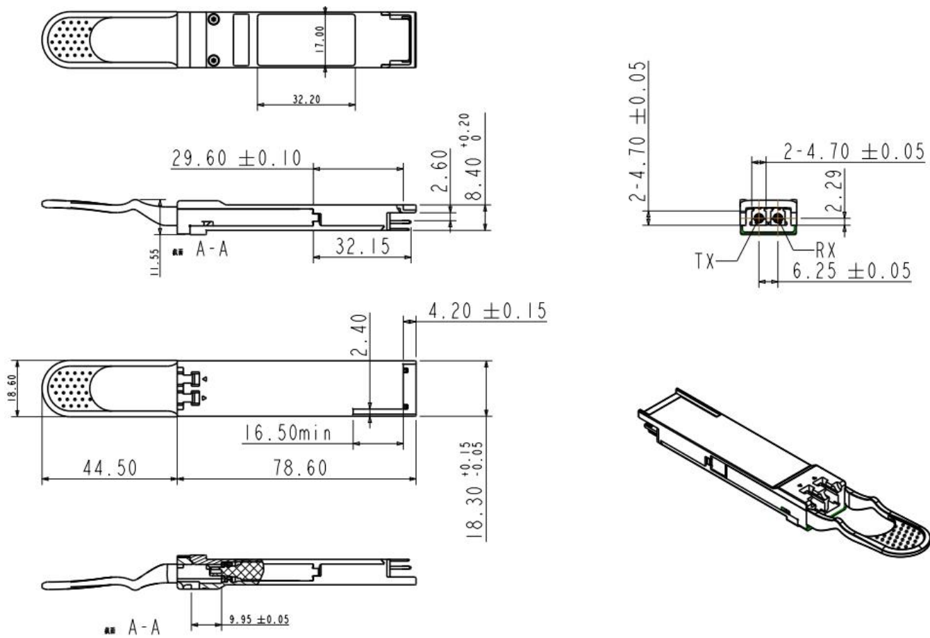
Figure 9. Mechanical Specifications
