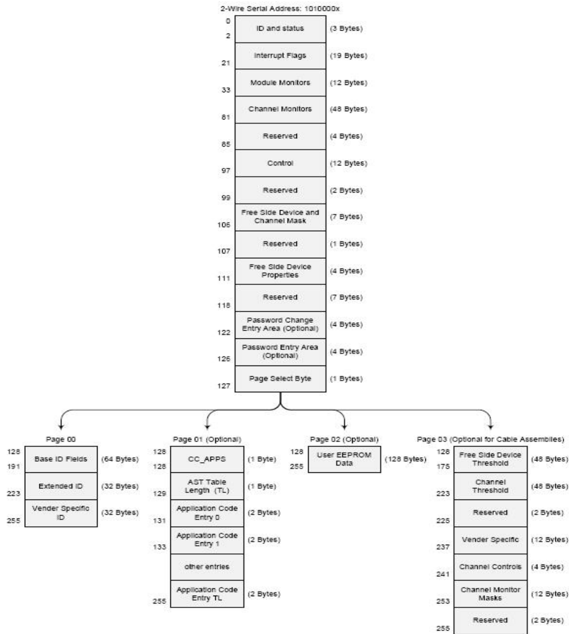
Figure5. QSF Memory Map
