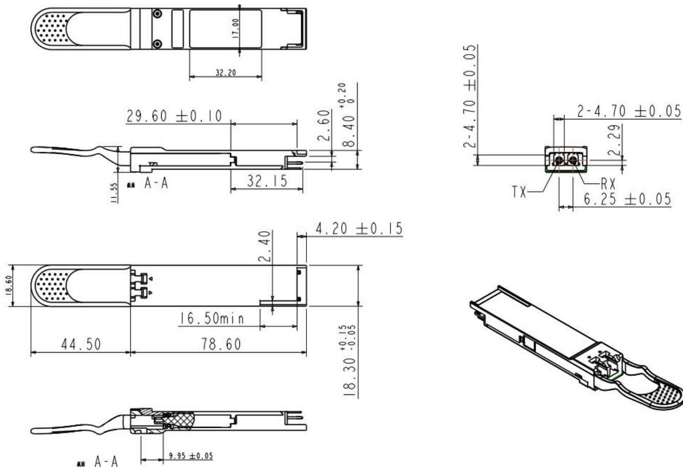
Figure 9 . Mechanical Specifications
