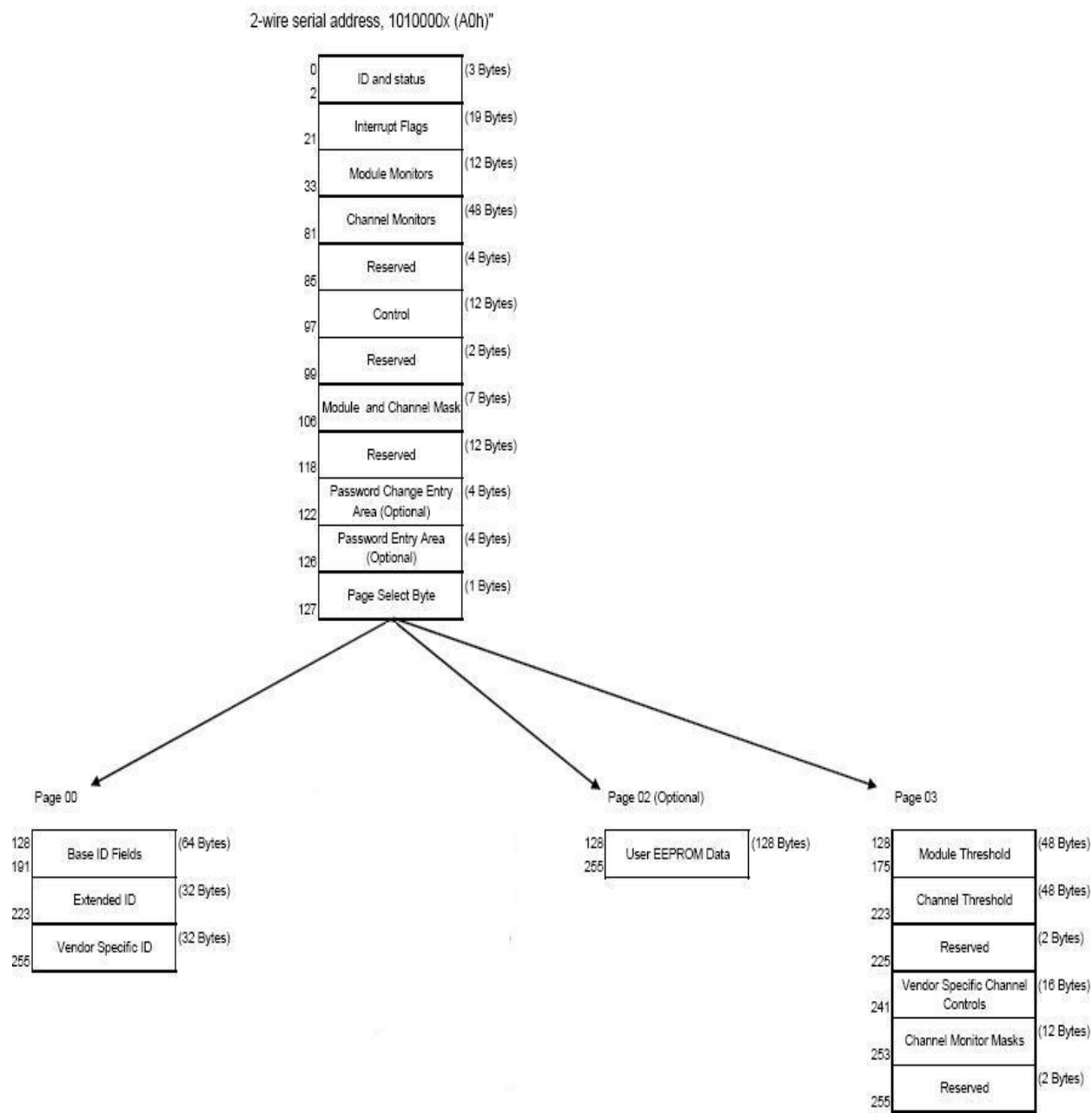
Figure5. QSFP Memory Map
