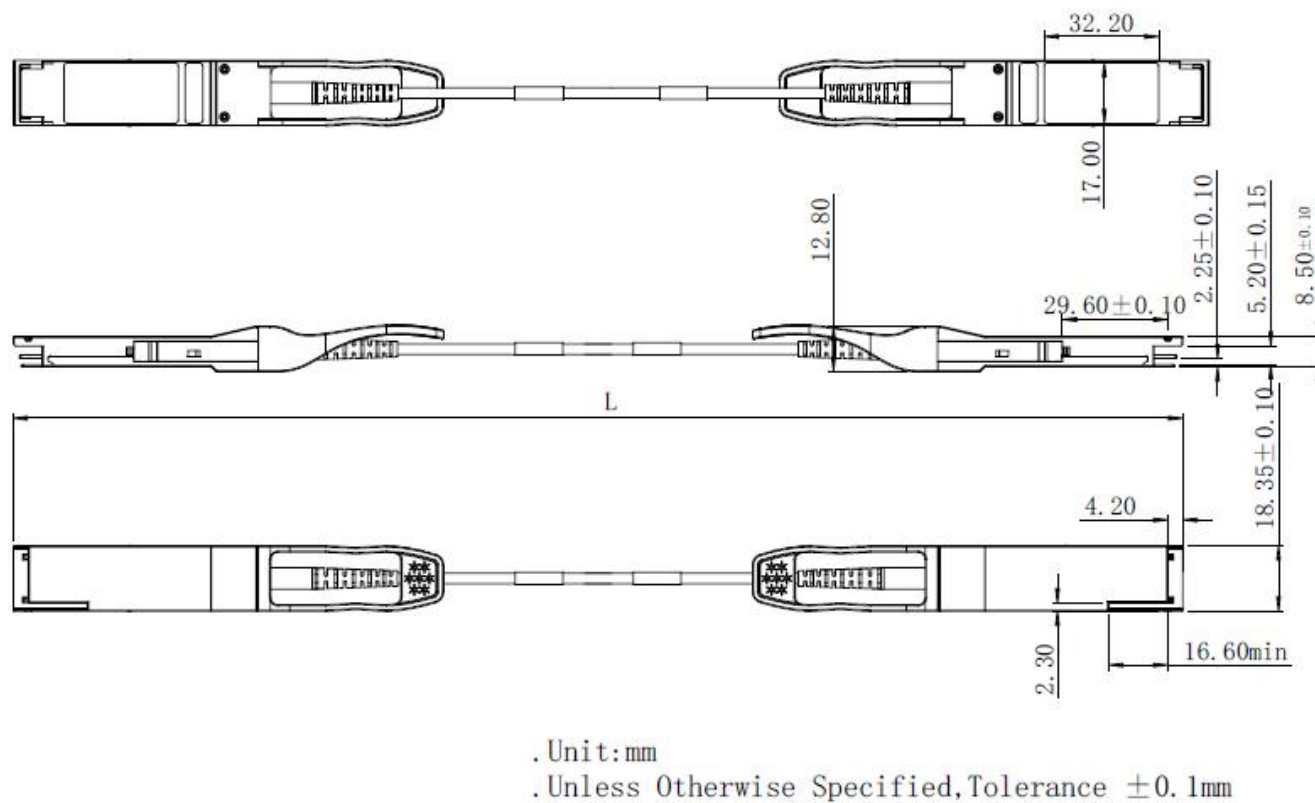
Figure9. Mechanical Specifications
