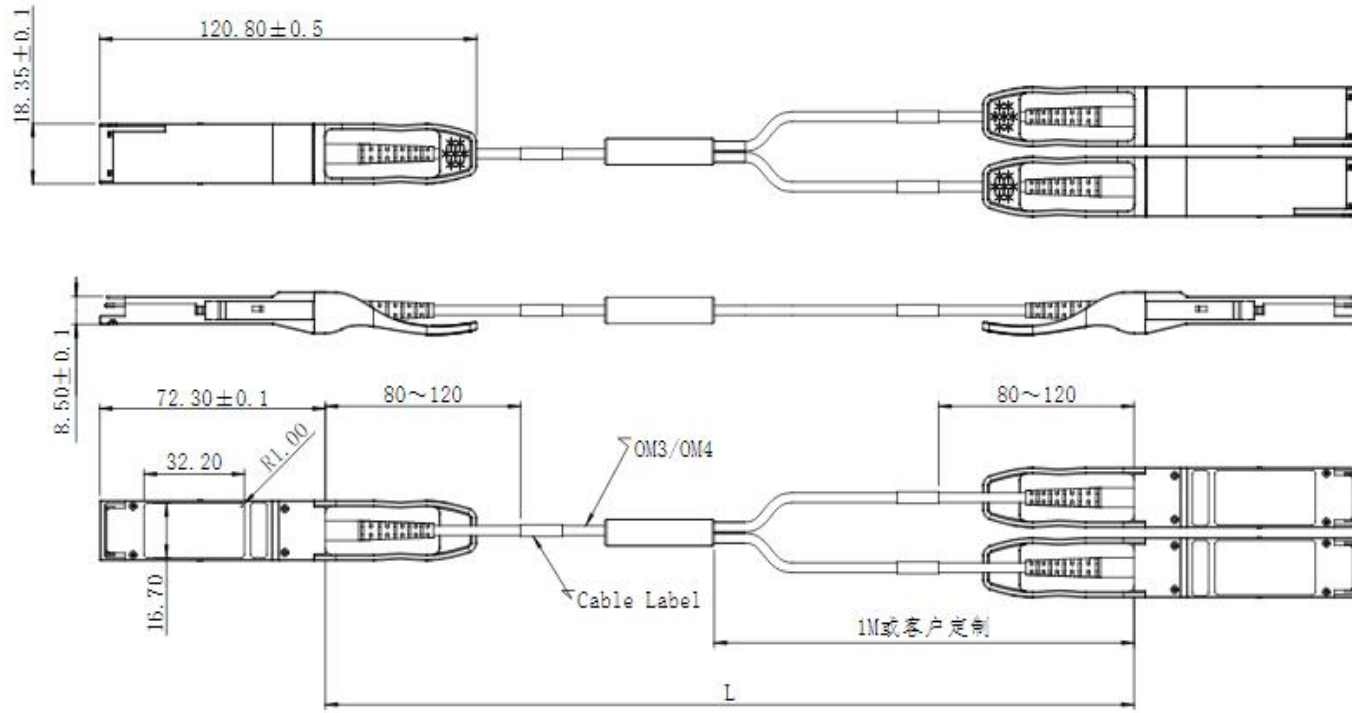
Figure 9. Mechanical Specifications
