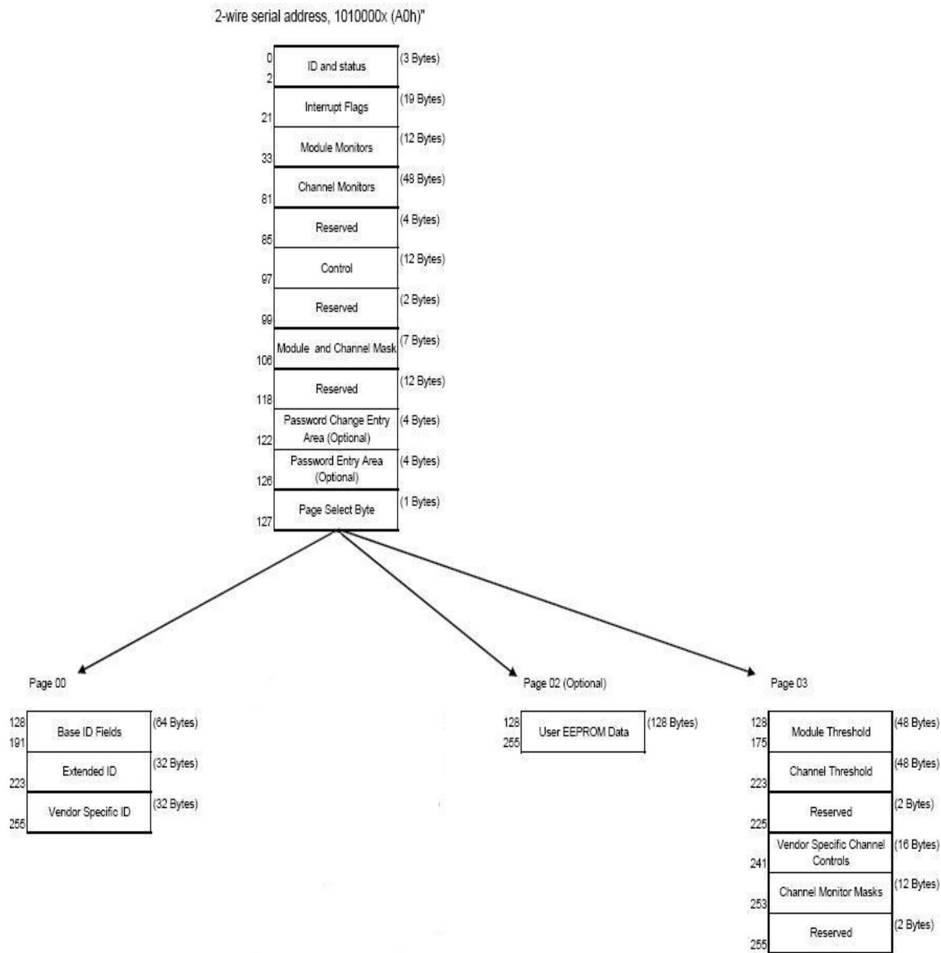
Figure5.QSFP Memory Map
