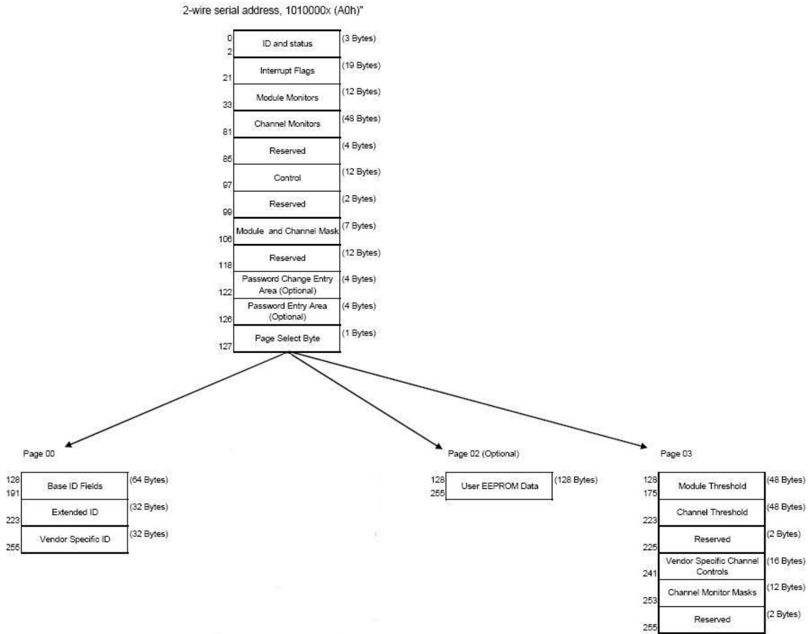
Figure 5. QSF Memory Map
