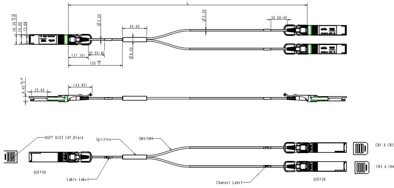
Figure 9. Mechanical Specifications
