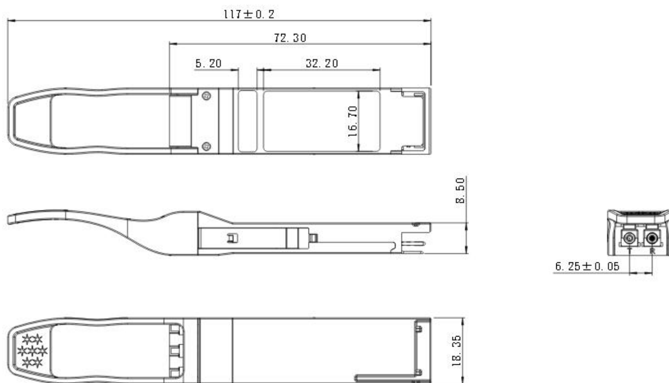
Figure 8. Mechanical Specifications
