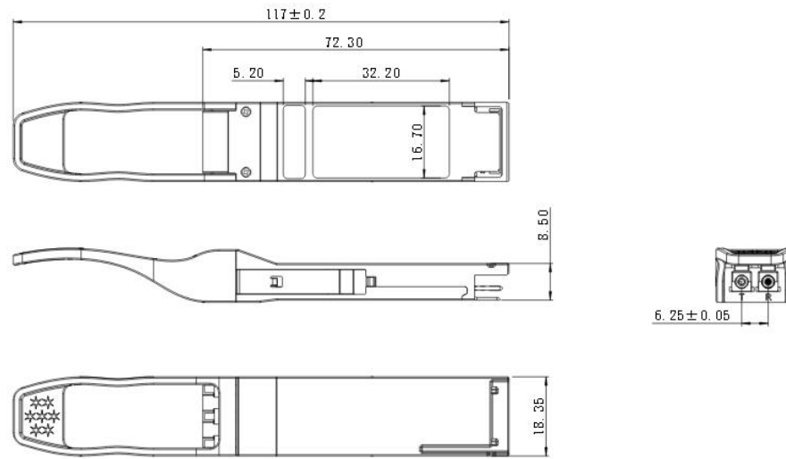
Figure 8. Mechanical Specifications
