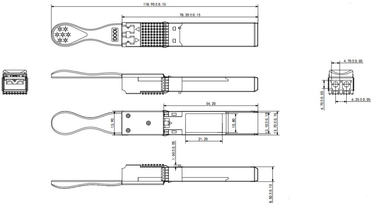
Figure 8. Mechanical Specifications
