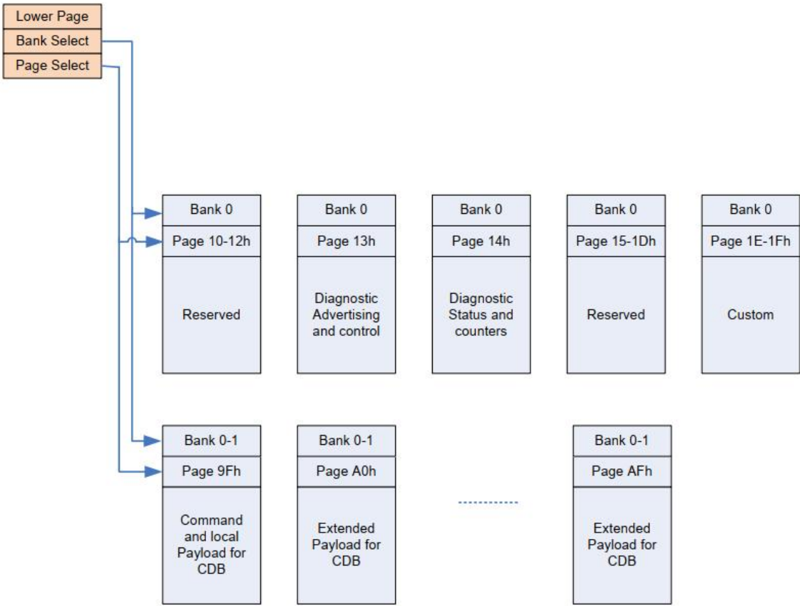
Figure 6. The Lower Memory Overview
