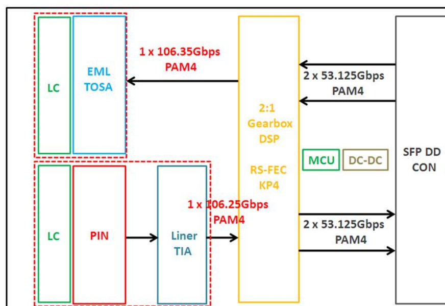
Figure 1. Module Block Diagram
