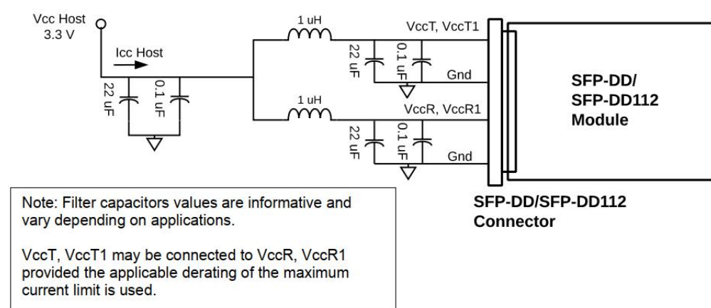
Figure 3. Host Board Power Supply Filtering
