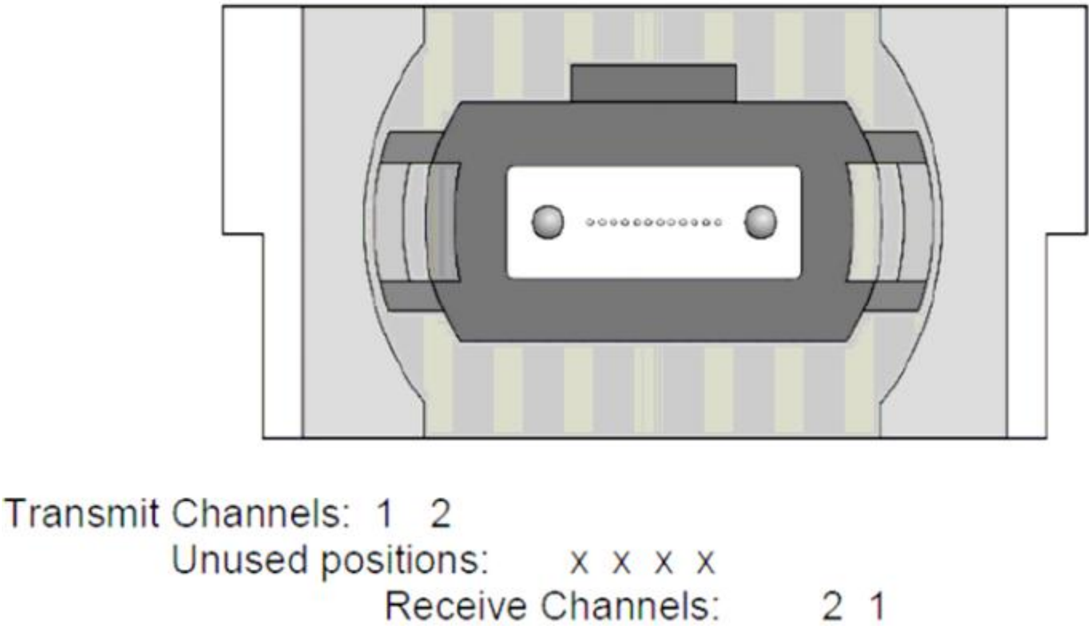
Figure 4. Optical Receptacle and Channel Orientation
