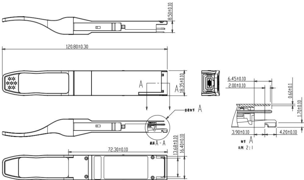
Figure 9. Mechanical Specifications
