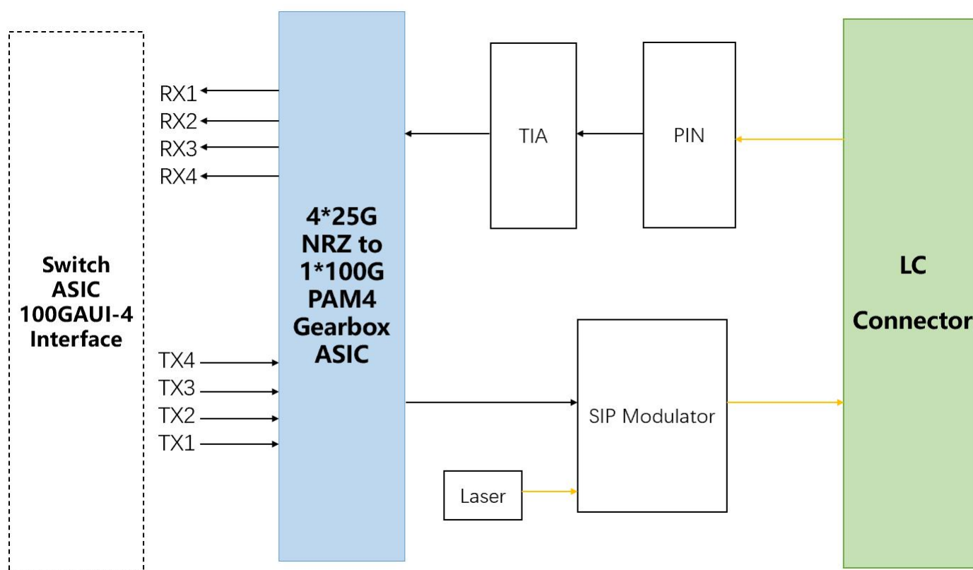
Figure 1. Module Block Diagram
