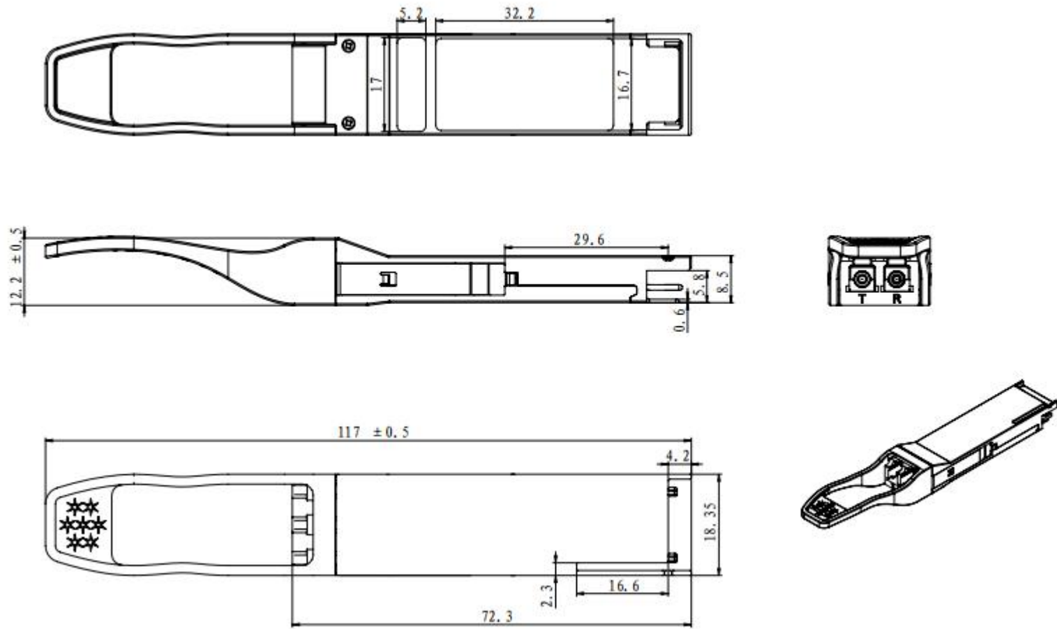
Figure 8. Mechanical Specifications
