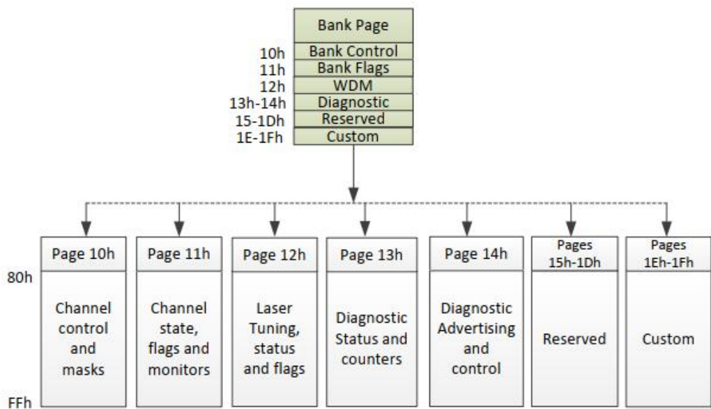
Figure 2. SFP112 Memory Map
