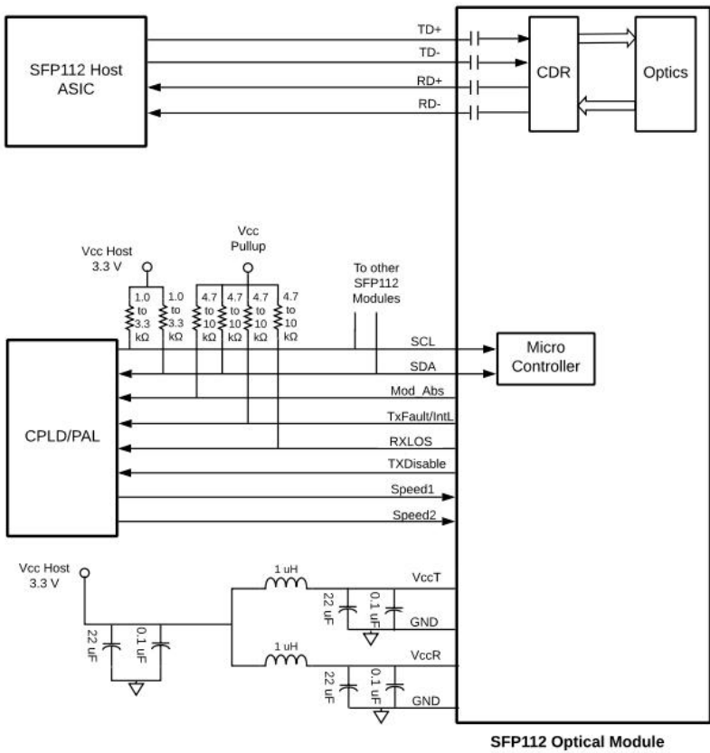
Figure5. Recommended Interface Circuit
