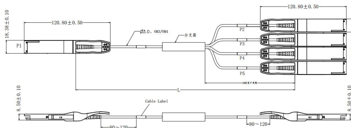
Figure 12. Mechanical Specifications
