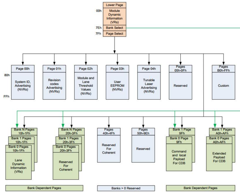
Figure 4. CMIS Bank Page Memory Map
